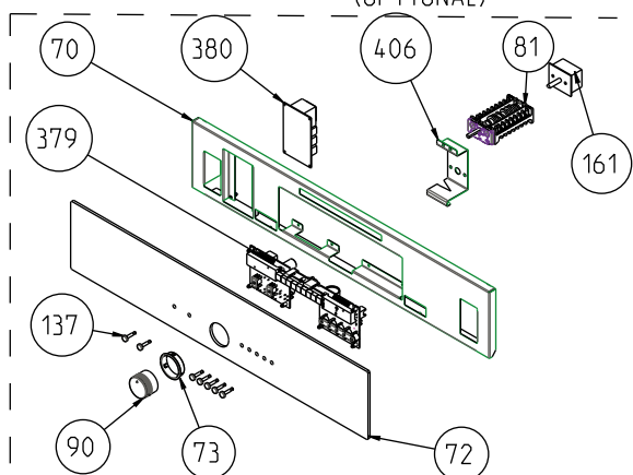
ELECTRONIC TIMERED GLASS CONTROL PANEL ASSEMBLY (OPTIONAL)
