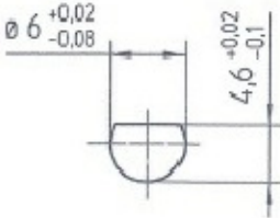
AXLE PROFILE
